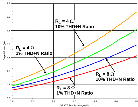
Figure 15. Output Power vs. VBATT - SD Mode
