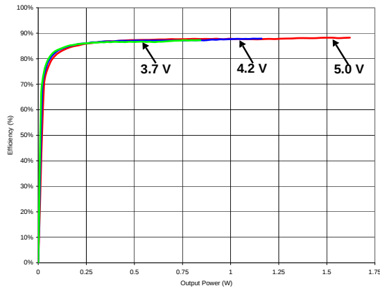
Figure 40. Efficiency vs. Output Power - HD Mode R_L = 8\ \Omega + 33\ \mu\text{H}
